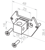
23 374.2501 16 x 16, Zapfen 22 mm
